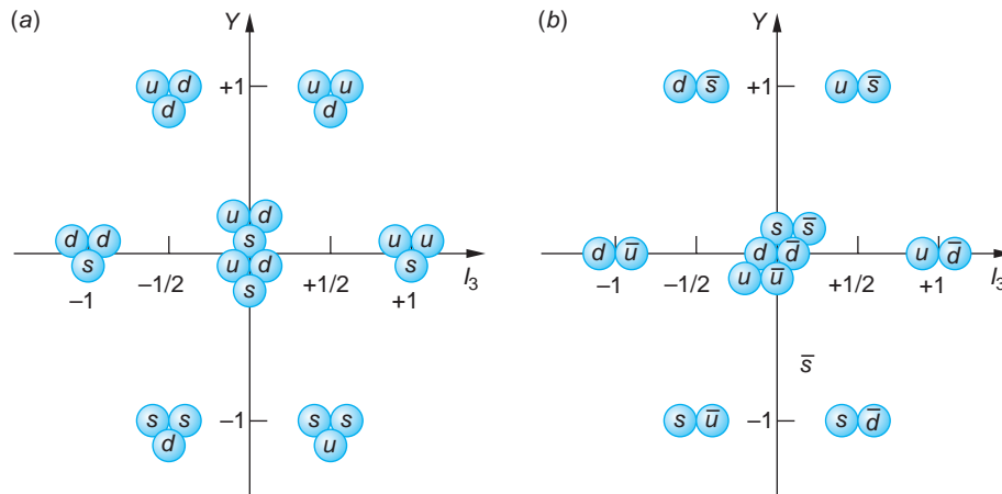
FIGURE 12-20 (a) The graph of Y versus I_3 for the spin-1/2 three-quark combinations—the baryon octet. (b) The graph of Y versus I_3 for the quark-antiquark combinations that form the lightest meson nonet.
